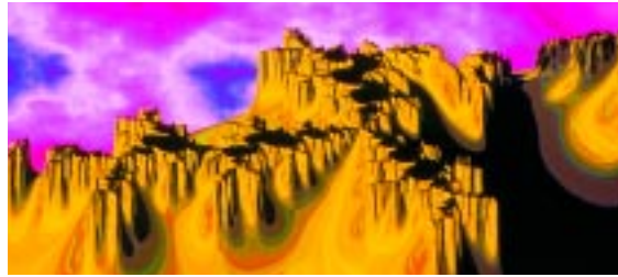
Fractal geometry of the sort used to generate these imaginary mountains can also model financial-market risk.
